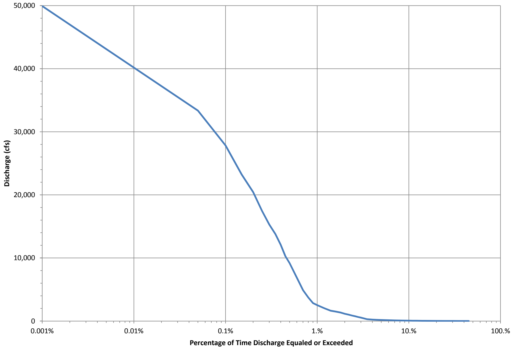
LPP Discharge-Duration Curve - LPP Alignment below Drain 30
