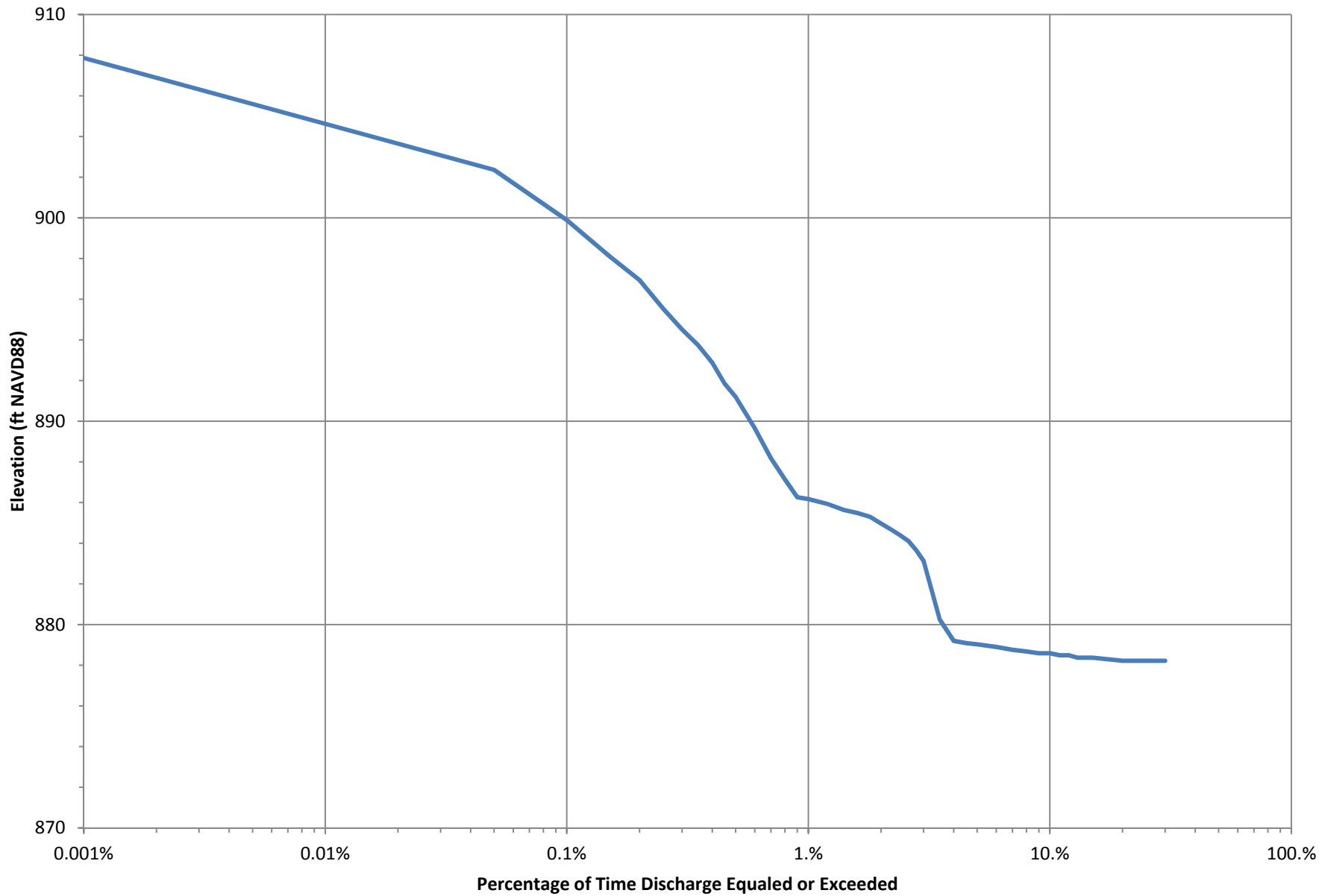
LPP Elevation-Duration Curve - LPP Alignment below Drain 21C
