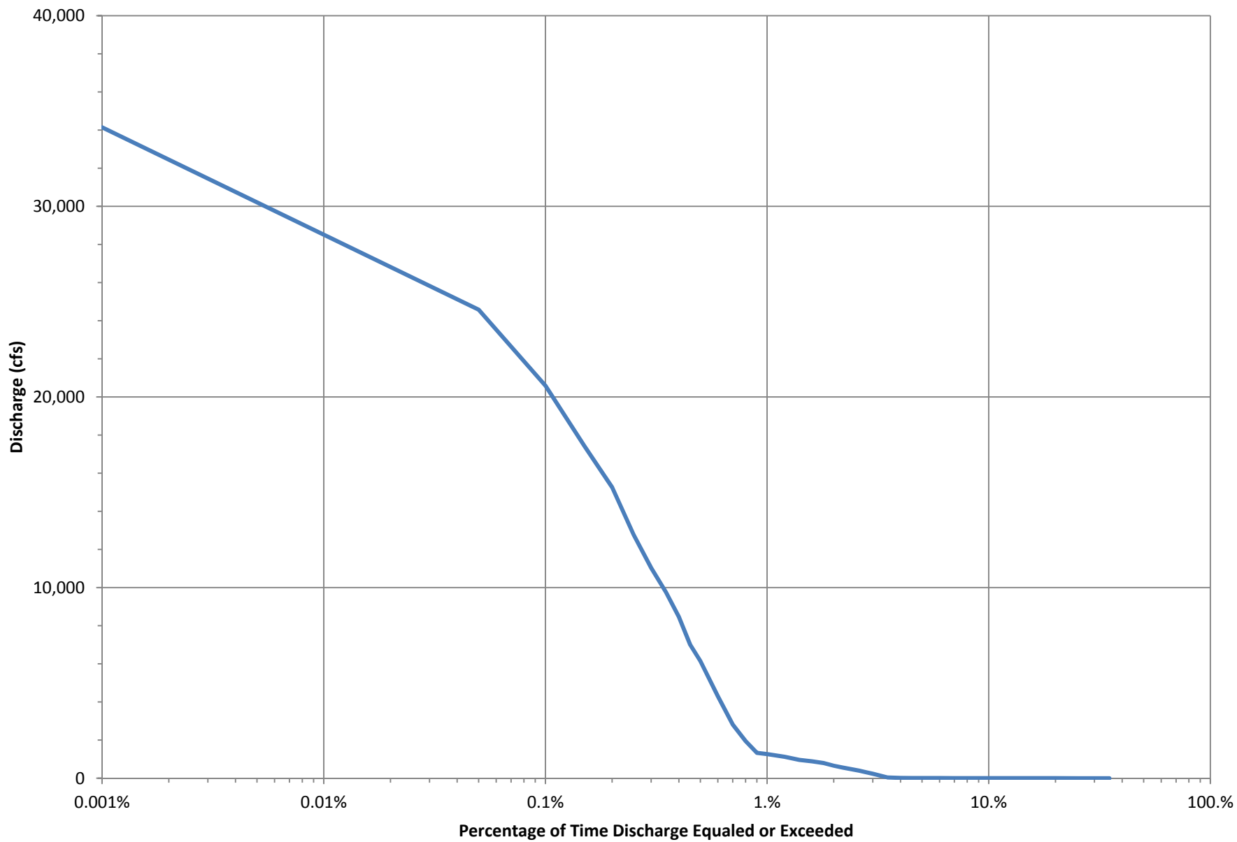
LPP Discharge-Duration Curve - LPP Alignment below Drain 21C
