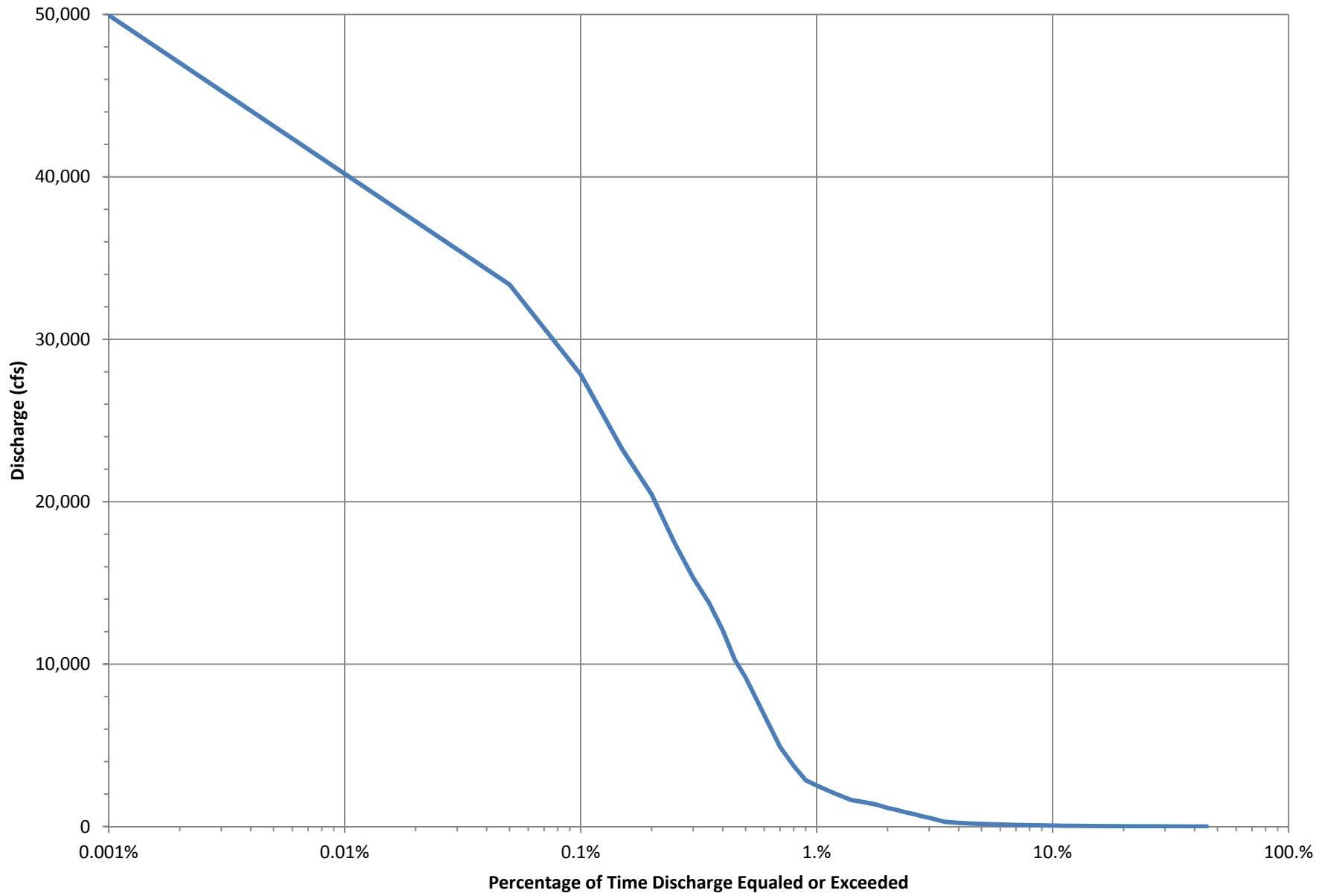
LPP Discharge-Duration Curve - LPP Alignment below Drain 29
