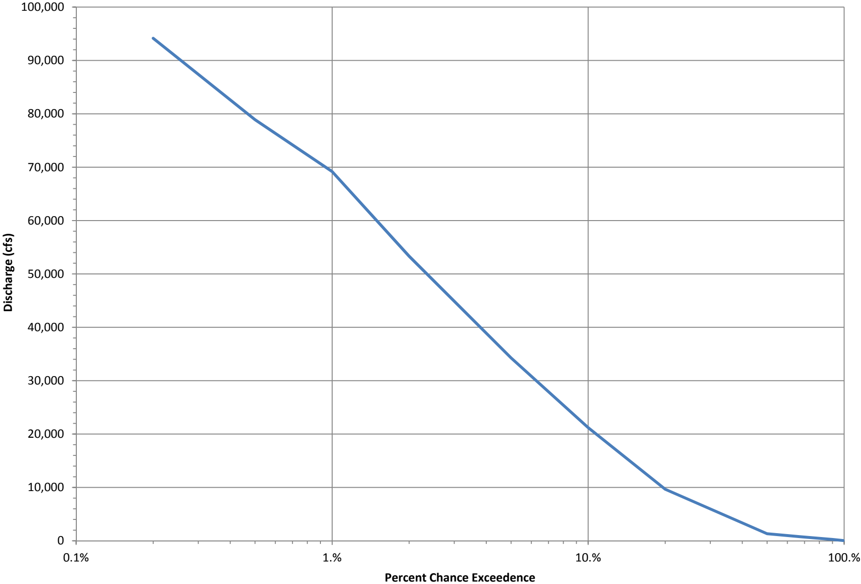
LPP Discharge-Frequency Curve - LPP Alignment below Drain 29
