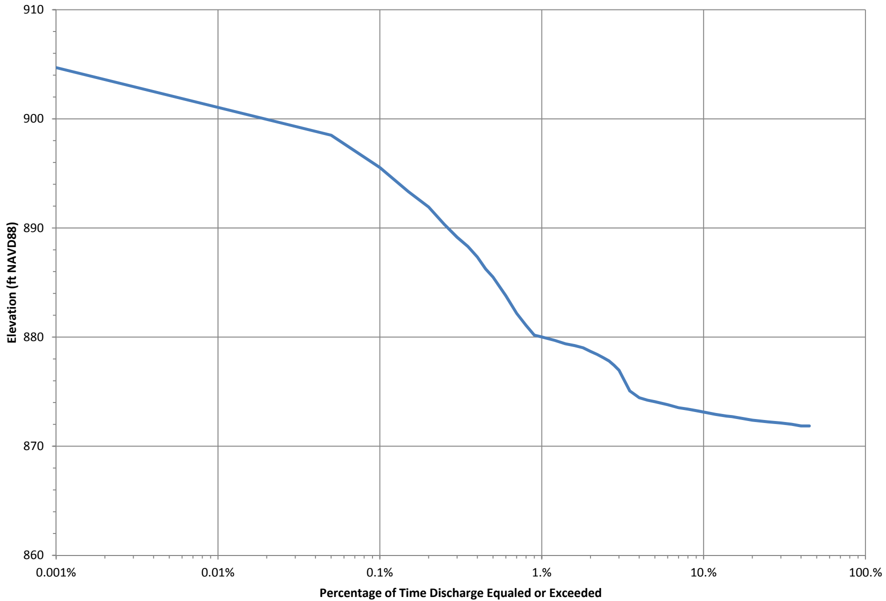
LPP Elevation-Duration Curve - LPP Alignment below Drain 14
