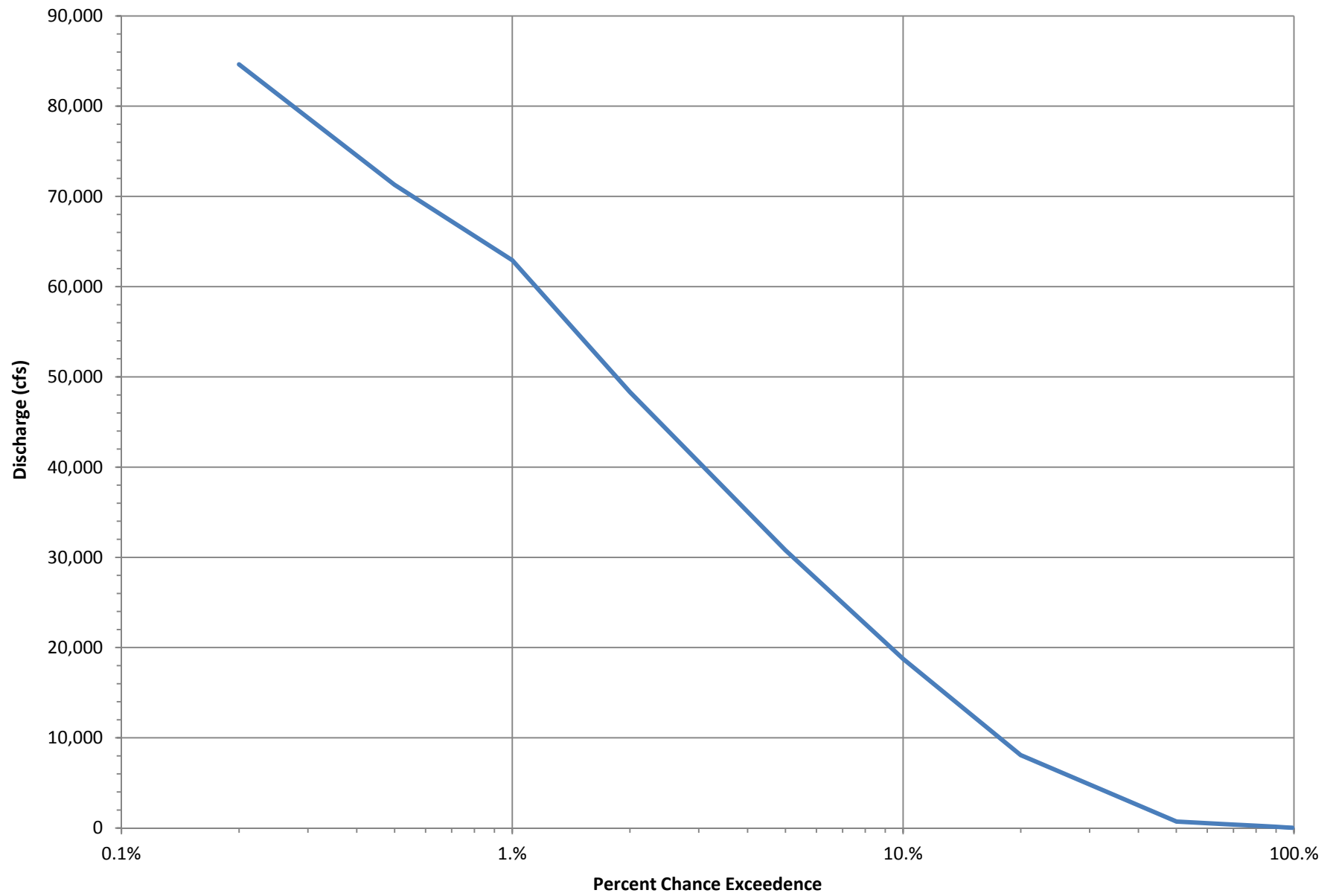
LPP Discharge-Frequency Curve - LPP Alignment below Lower Rush River
