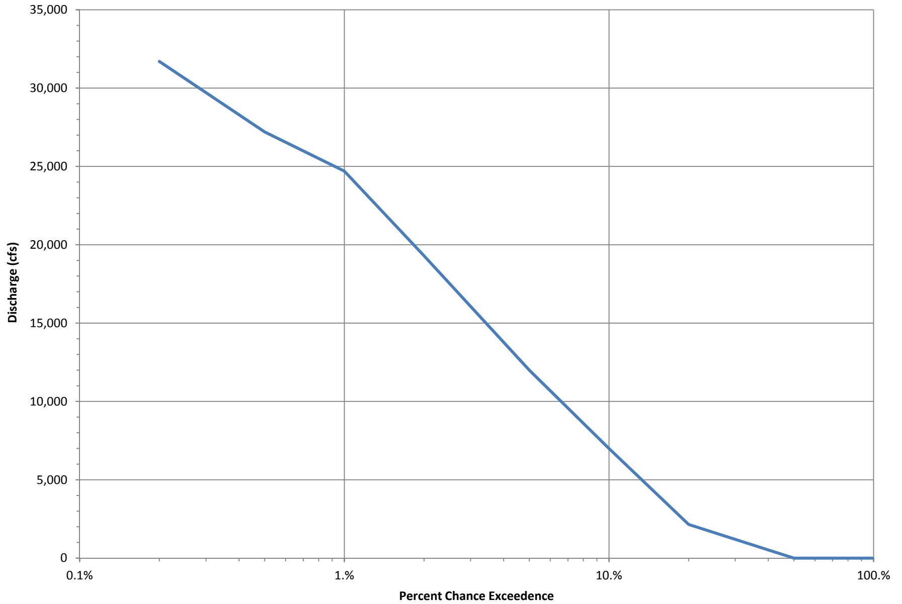
LPP Discharge-Frequency Curve - LPP Alignment below Red River
