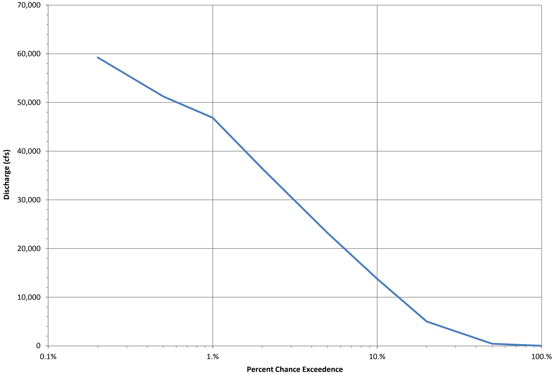
LPP Discharge-Frequency Curve - LPP Alignment below Drain 14
