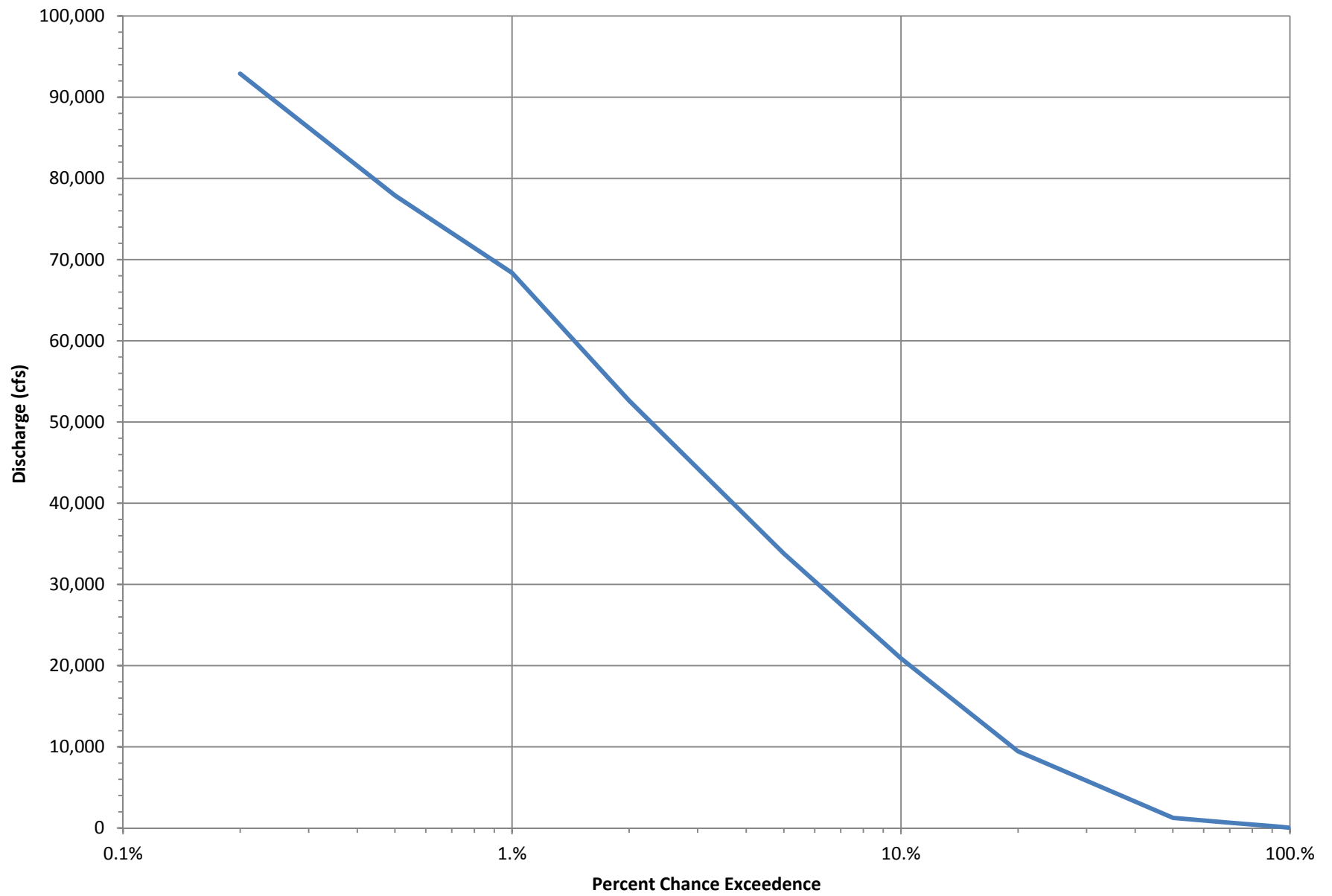
LPP Discharge-Frequency Curve - LPP Alignment below Rush River
