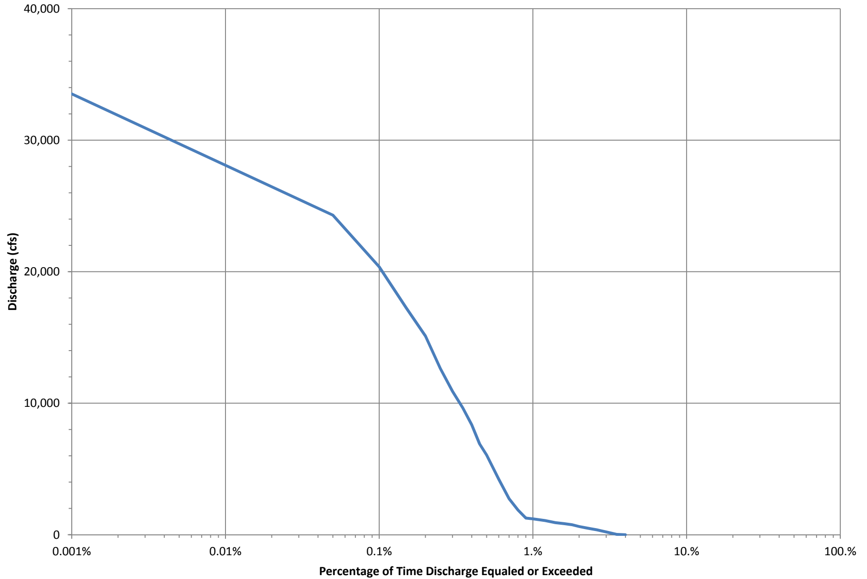
LPP Discharge-Duration Curve - LPP Alignment below Sheyenne River
