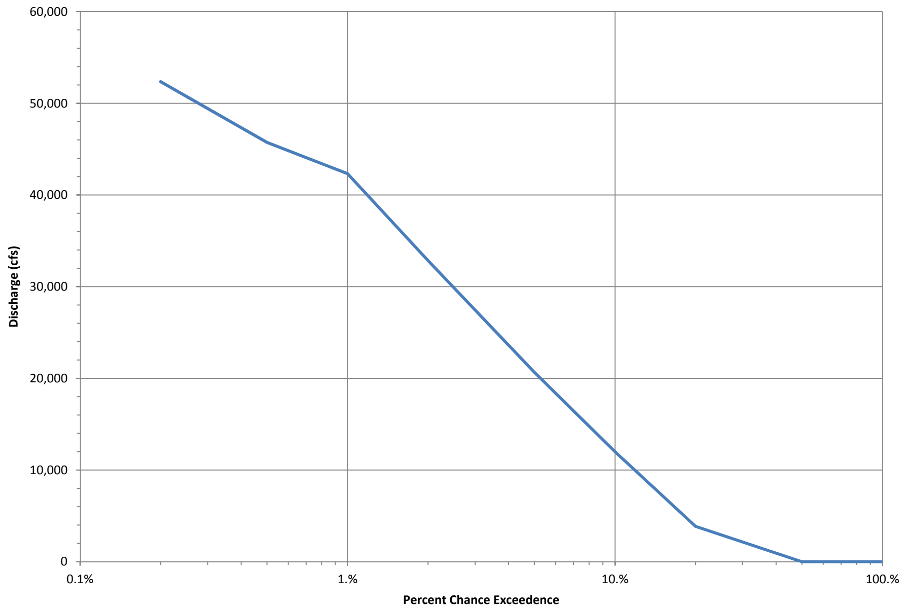
LPP Discharge-Frequency Curve - LPP Alignment below Sheyenne River
