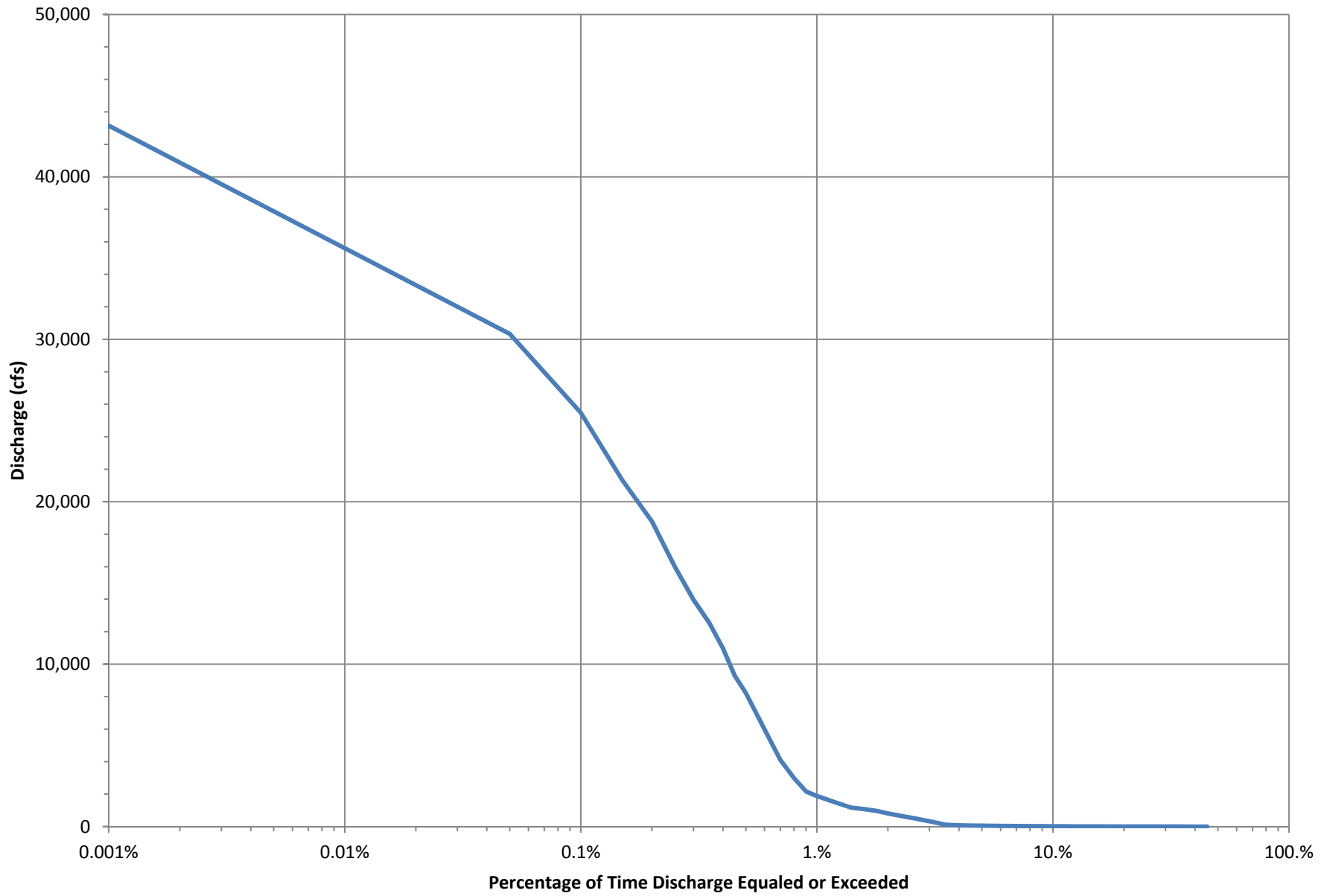
LPP Discharge-Duration Curve - LPP Alignment below Maple River
