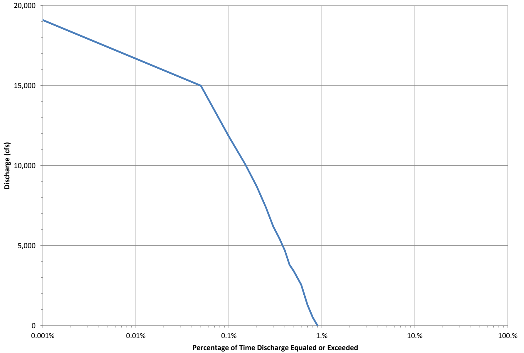
LPP Discharge-Duration Curve - LPP Alignment below Red River
