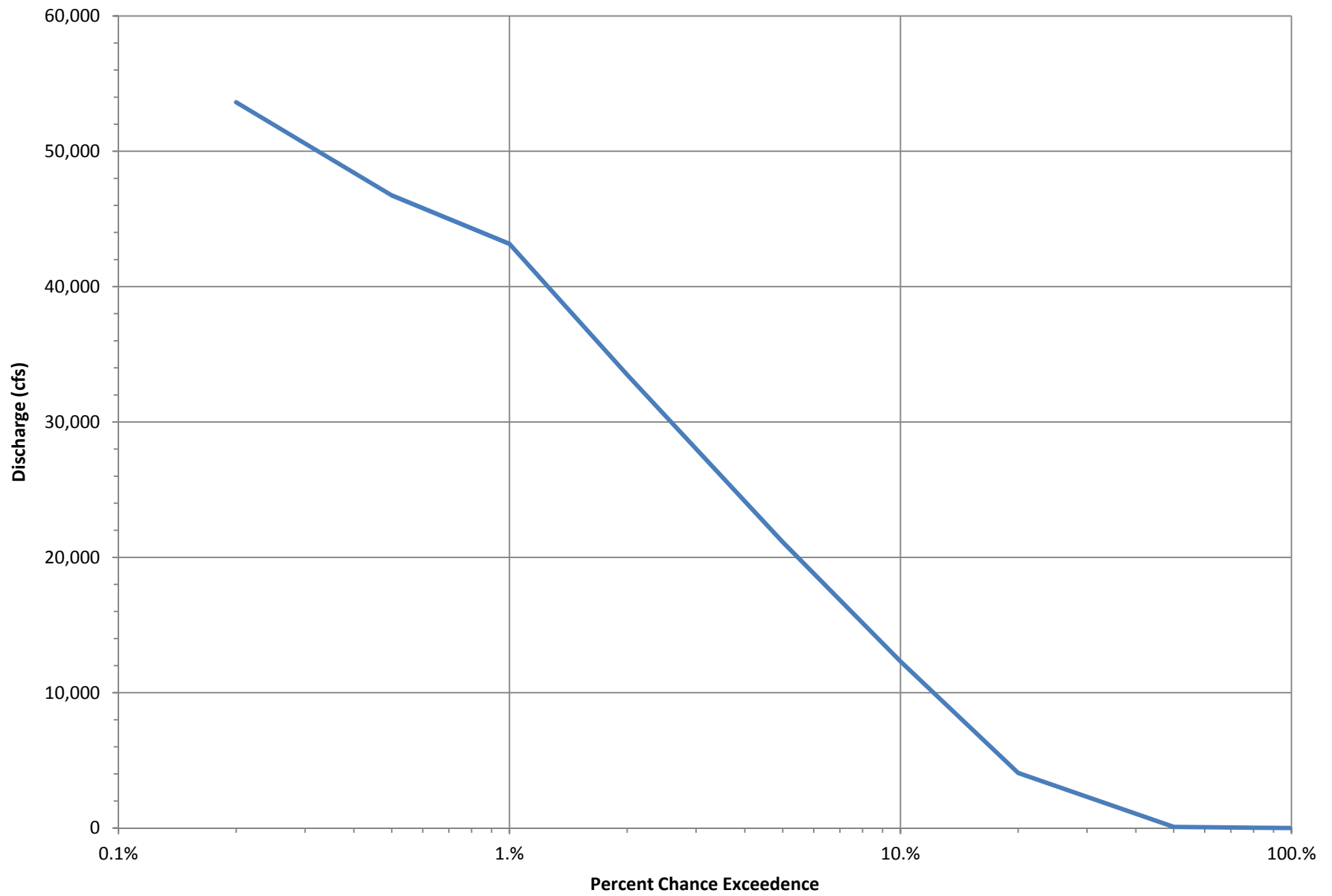
LPP Discharge-Frequency Curve - LPP Alignment below Drain 21C
