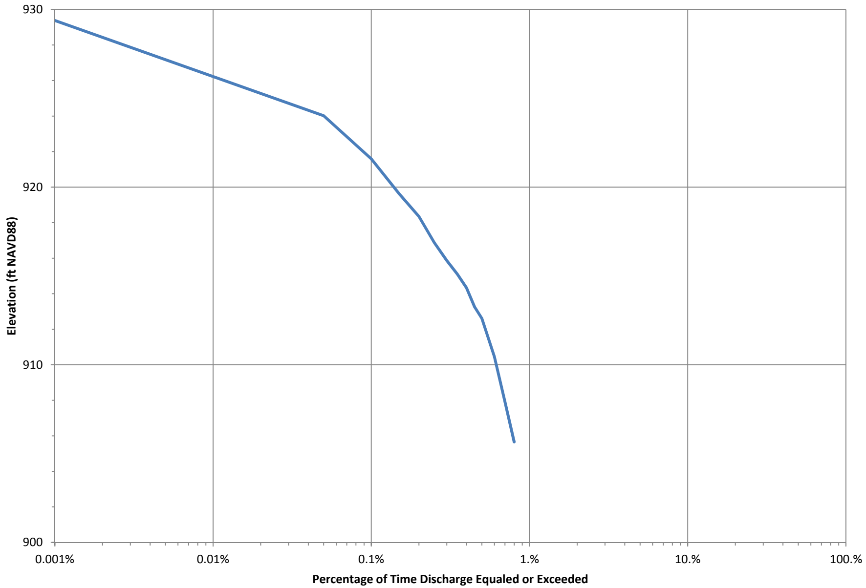
LPP Elevation-Duration Curve - LPP Alignment below Wild Rice River
