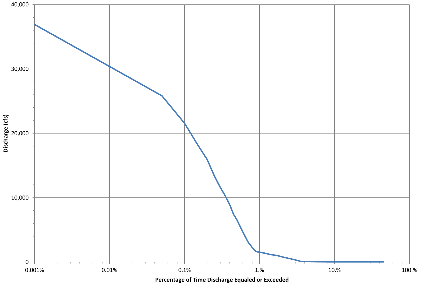
LPP Discharge-Duration Curve - LPP Alignment below Drain 14
