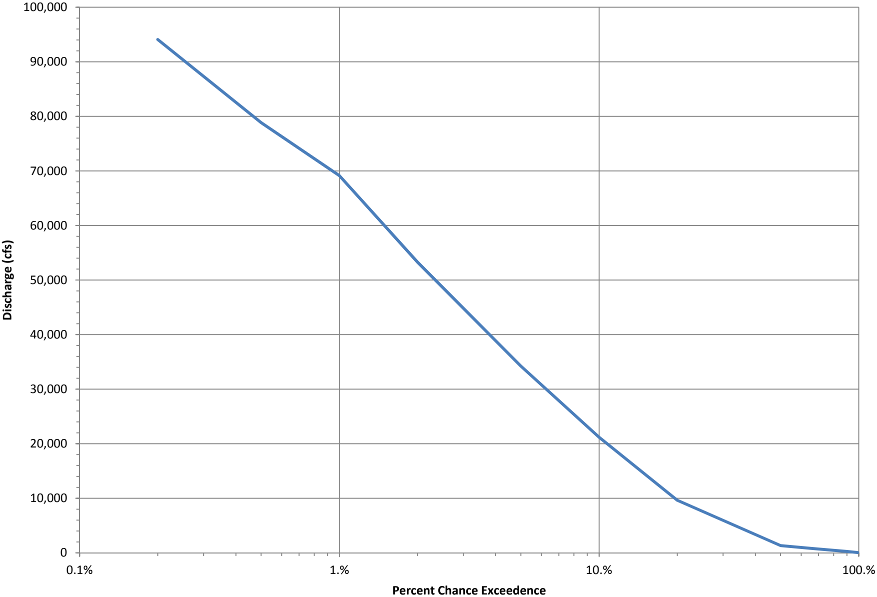
LPP Discharge-Frequency Curve - LPP Alignment below Drain 30
