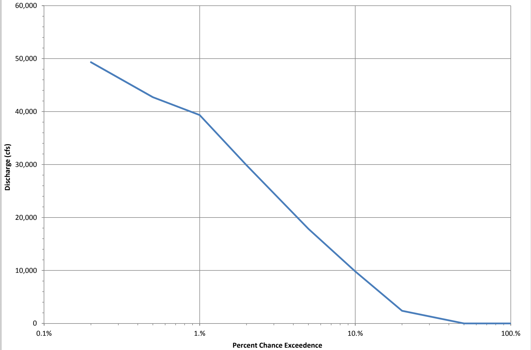
LPP Discharge-Frequency Curve - LPP Alignment below Wild Rice River
