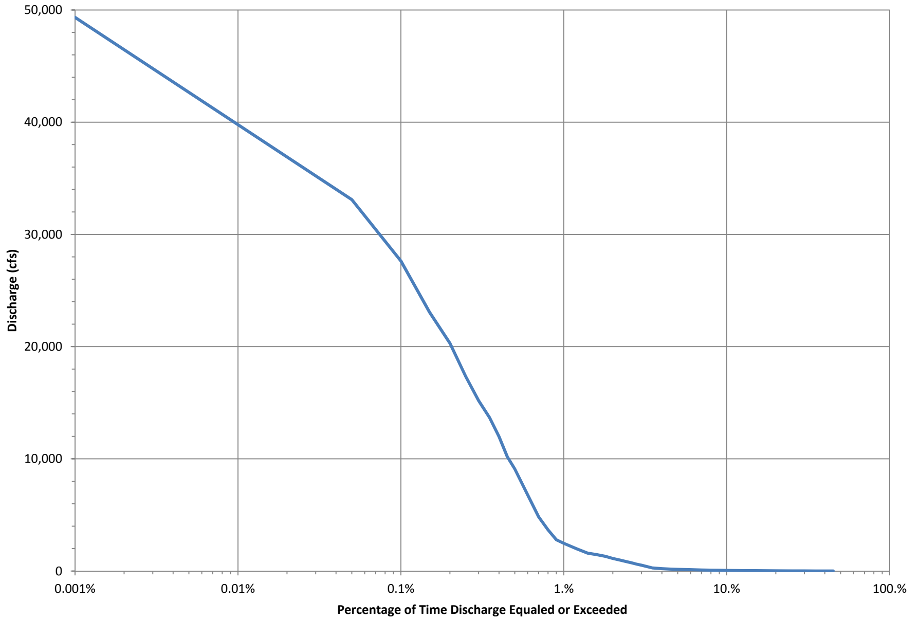
LPP Discharge-Duration Curve - LPP Alignment below Rush River
