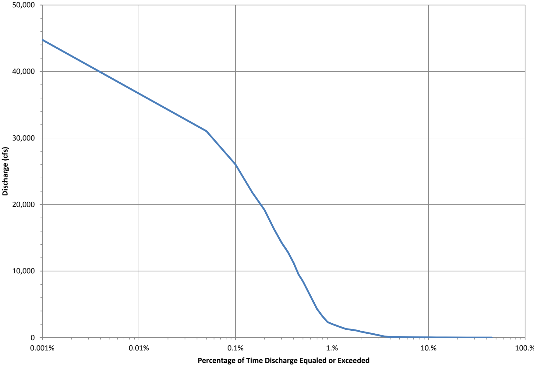
LPP Discharge-Duration Curve - LPP Alignment below Lower Rush River
